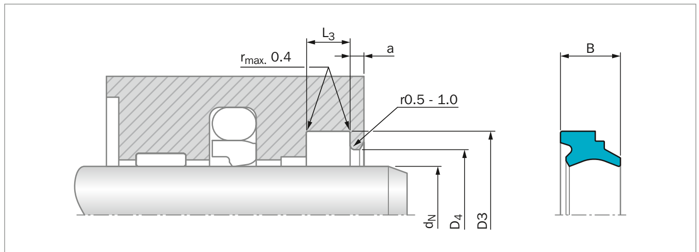
Figure 180: Installation Drawing
