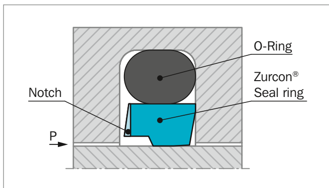
Figure 27: Zurcon® Rimseal
