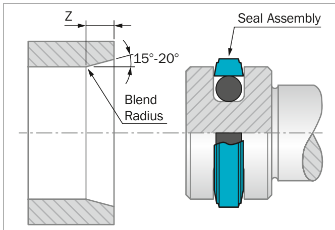
Figure 95: Lead-in chamfer
