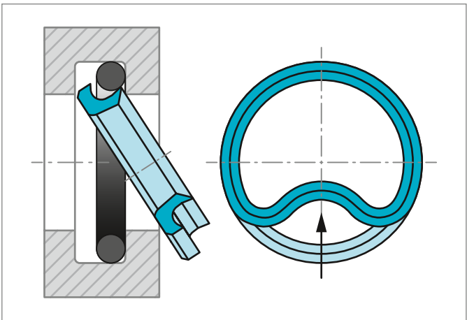
Figure 11: Installation of Rod VL Seal® in closed groove
