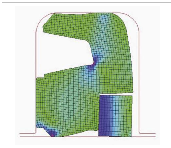
Figure 64: Pressure relief with a back pressure bigger of 0.5 MPa (72.5 psi)
