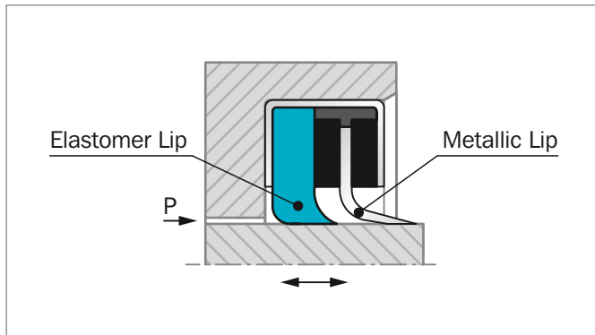
Figure 198: Metal Scraper
