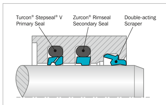
Figure 25: Turcon® Stepseal® 2K and Zurcon® Rimseal in tandem configuration
