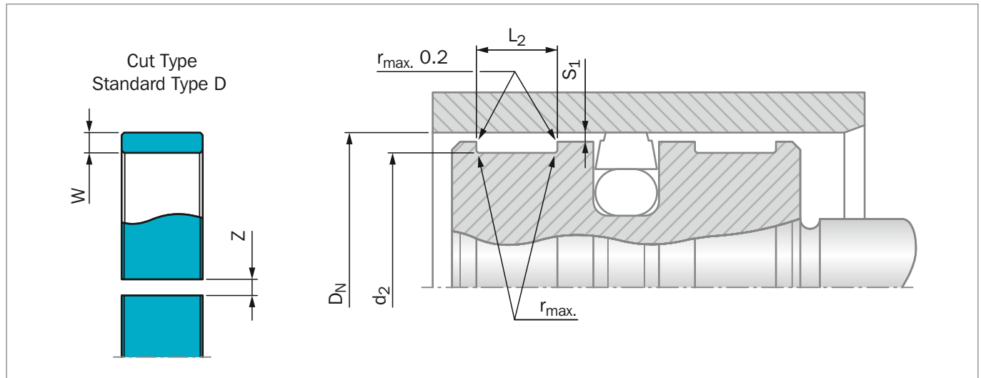
Figure 214: Installation Drawing
