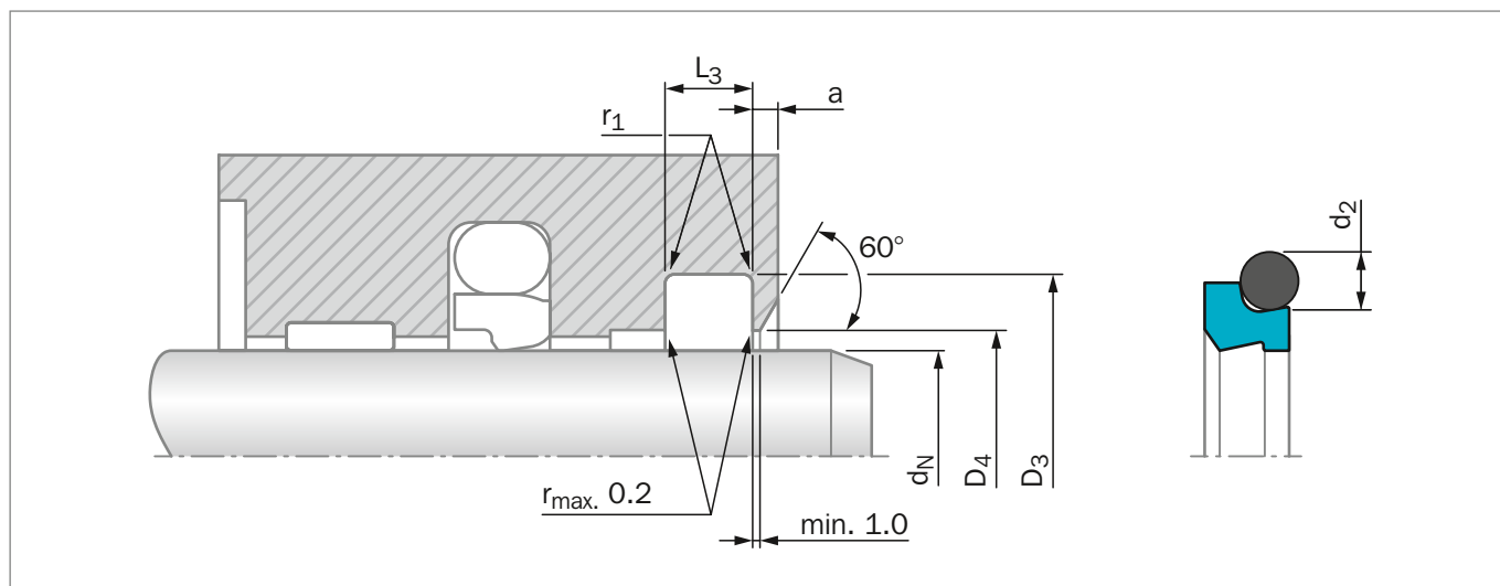
Figure 165: Installation Drawing
