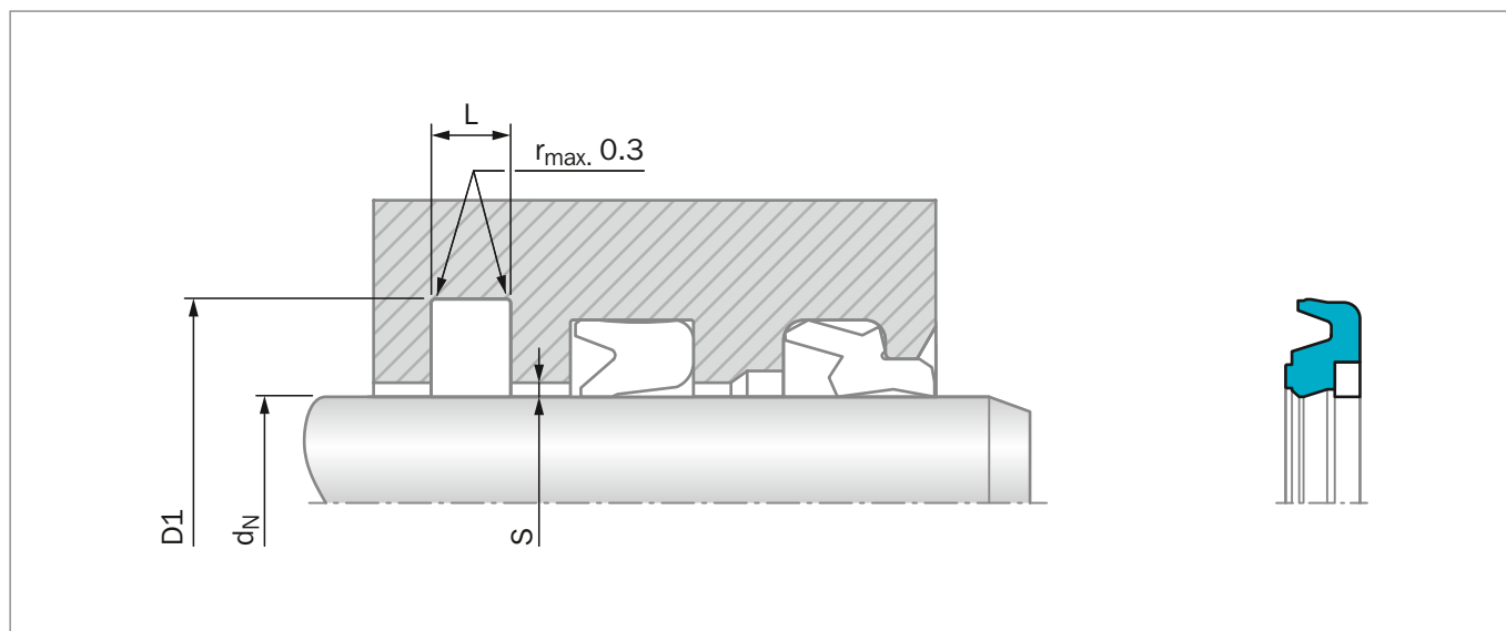
Figure 65: Installation Drawing
