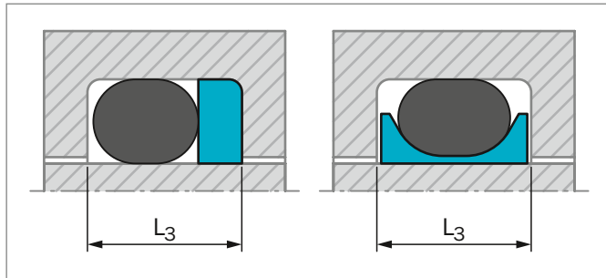
Figure 94: Groove width
