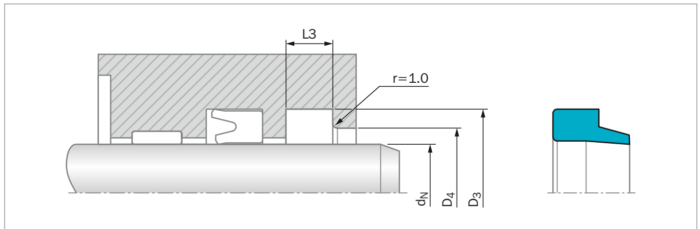
Figure 187: Installation Drawing
