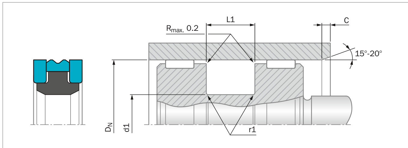
Figure 149: Installation Drawing
