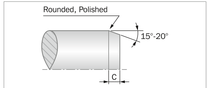
Figure 46: Lead-in chamfer
