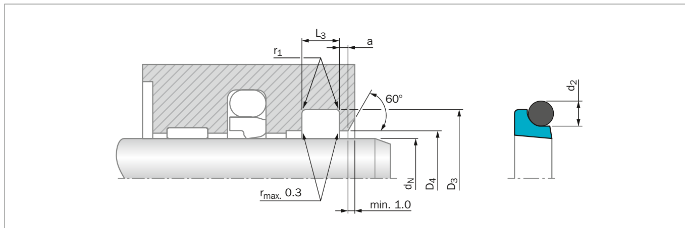
Figure 176: Installation Drawing
