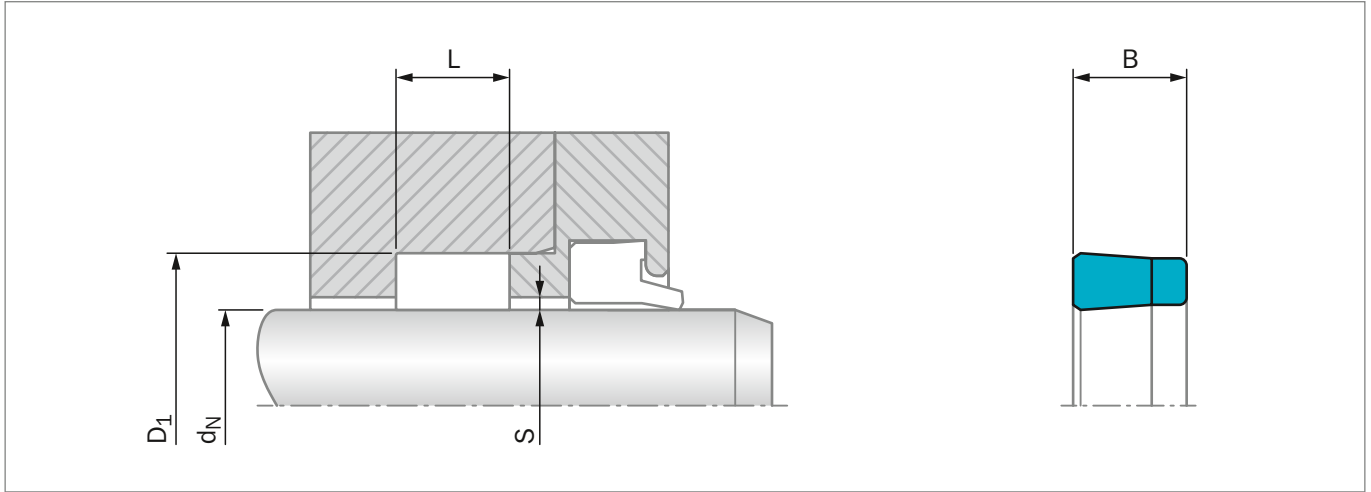
Figure 40: Installation Drawing
