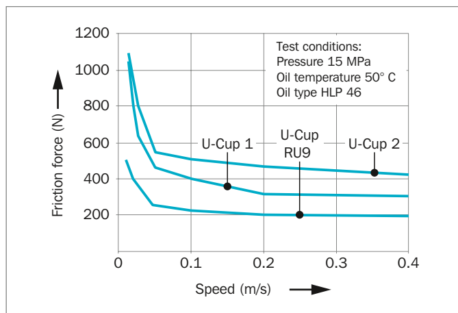
Figure 55: Friction dependent on speed
