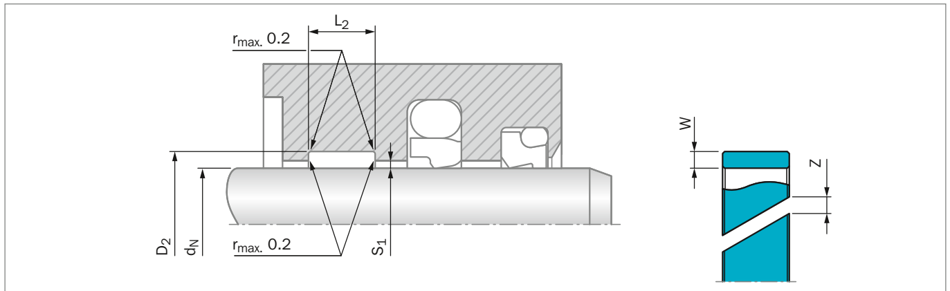
Figure 212: Installation Drawing
