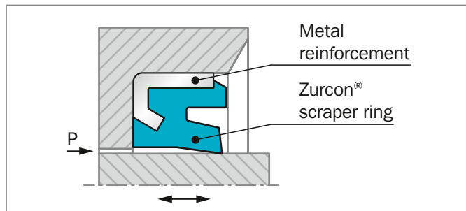
Figure 196: Scraper SWP
