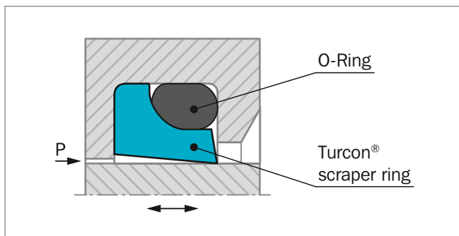
Figure 174: Turcon® Excluder® 1 an all-round single acting scraper
