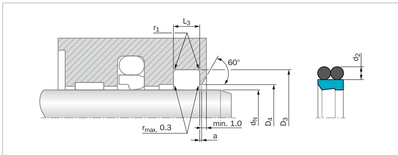
Figure 167: Installation Drawing
