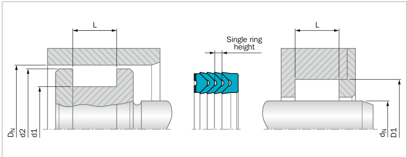
Figure 33: Installation Drawing
