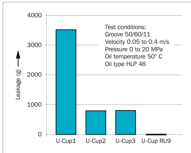
Figure 57: Leakage performance dependent on U-Cup type
