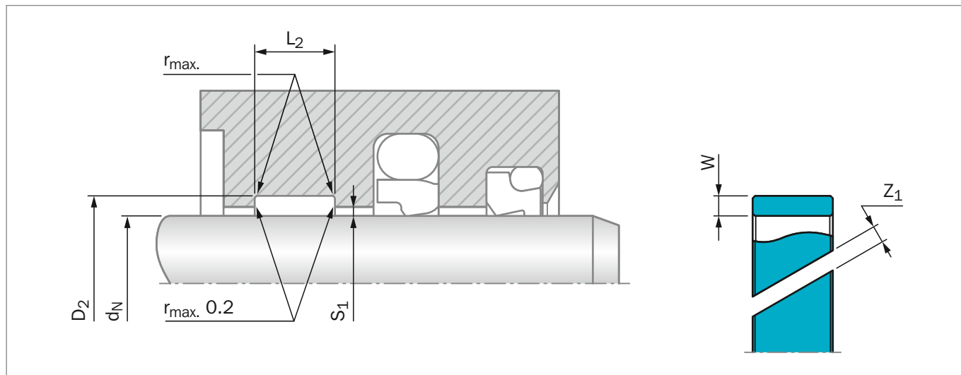
Figure 215: Installation Drawing
