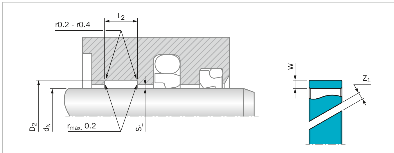
Figure 220: Installation Drawing
