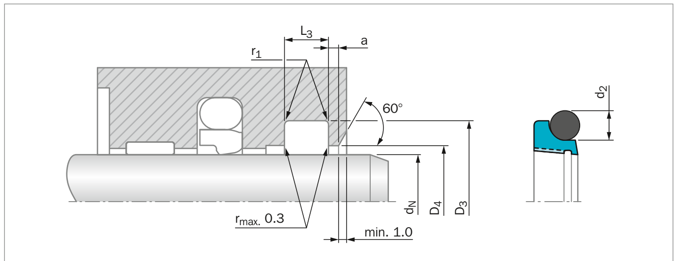
Figure 178: Installation Drawing
