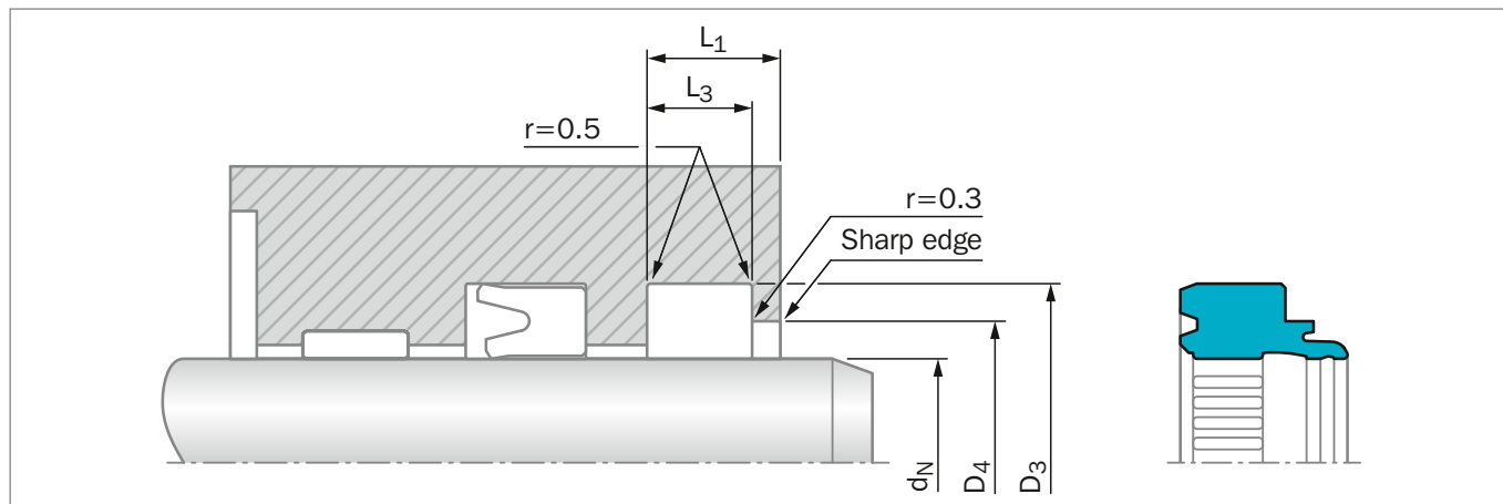
Figure 193: Installation Drawing
