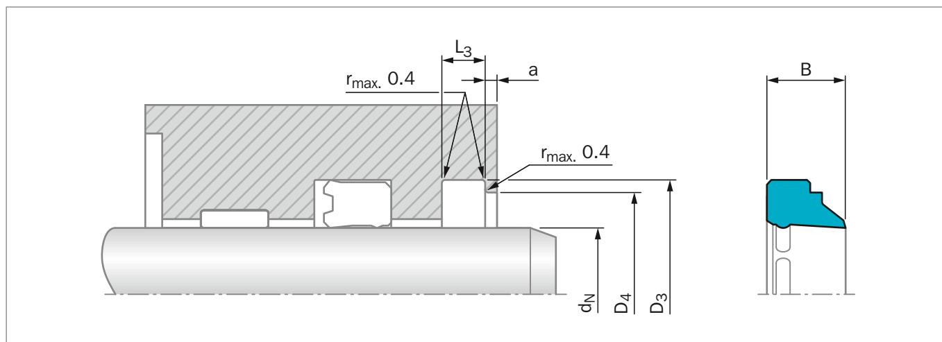
Figure 189: Installation Drawing
