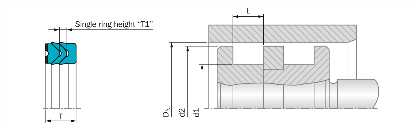
Figure 159: Installation Drawing
