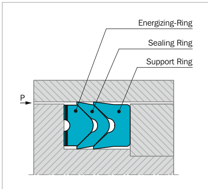
Figure 158: Veepac CH/G1
