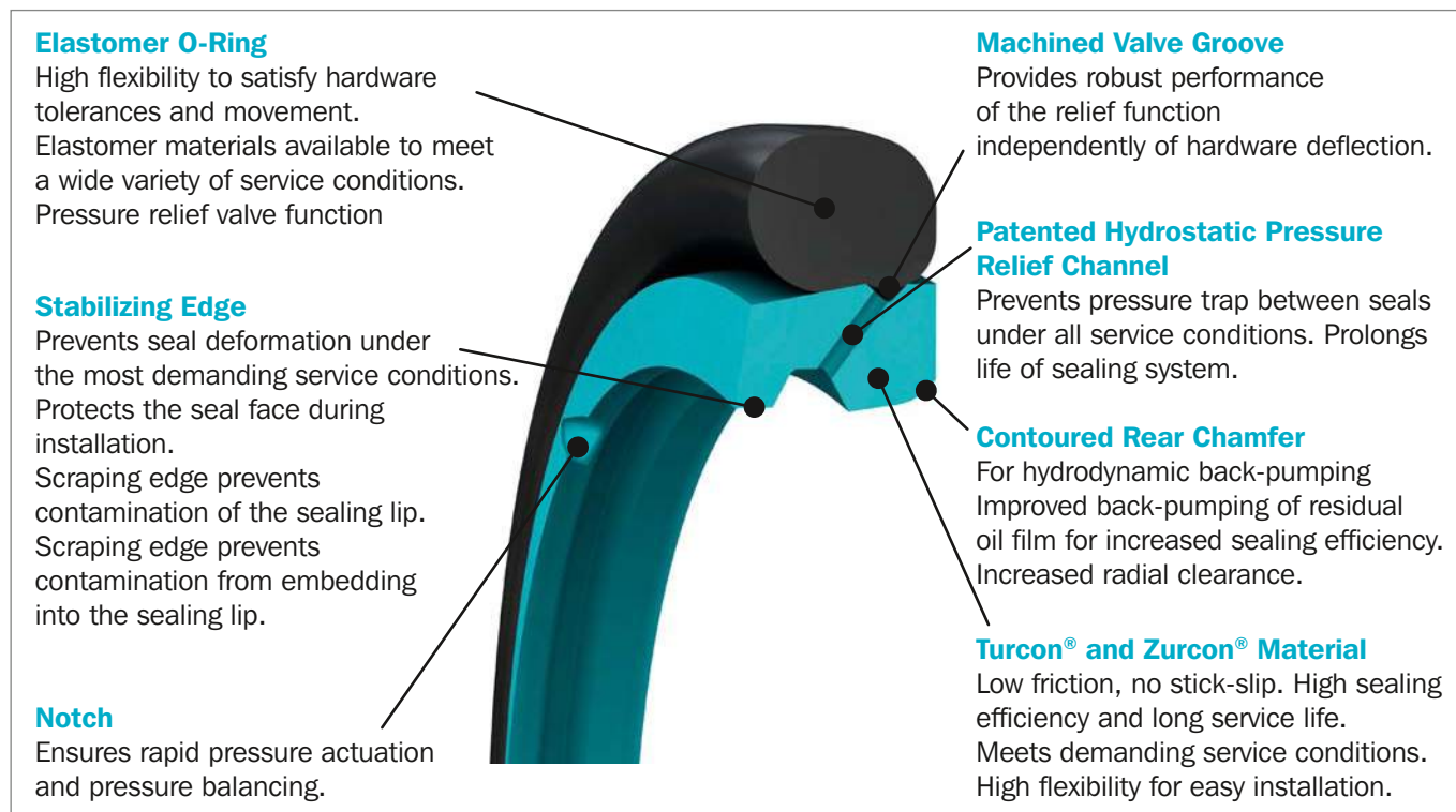
Figure 24: Turcon® Stepseal® V design features
