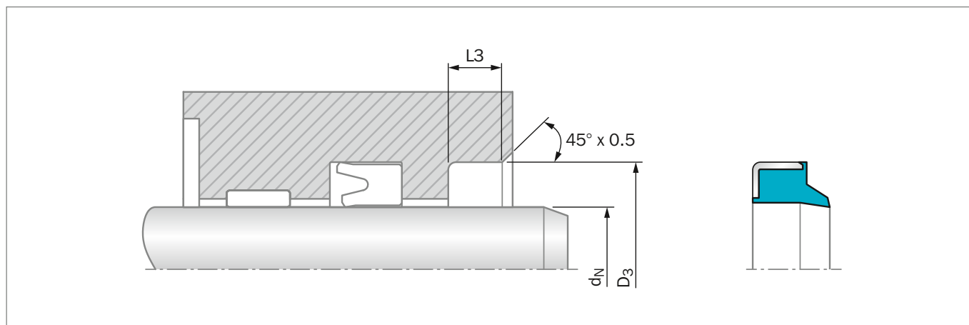
Figure 195: Installation Drawing
