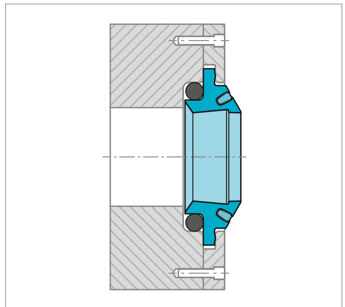
Figure 170: Turcon® Excluder® S installed in split groove
