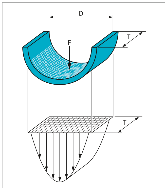
Figure 204: Load distribution
