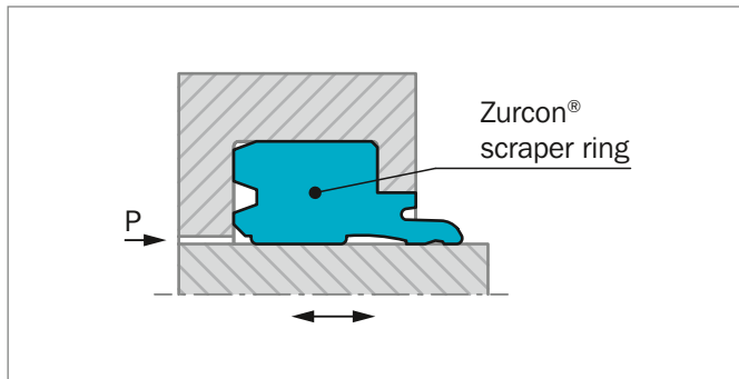
Figure 192: Scraper WNV
