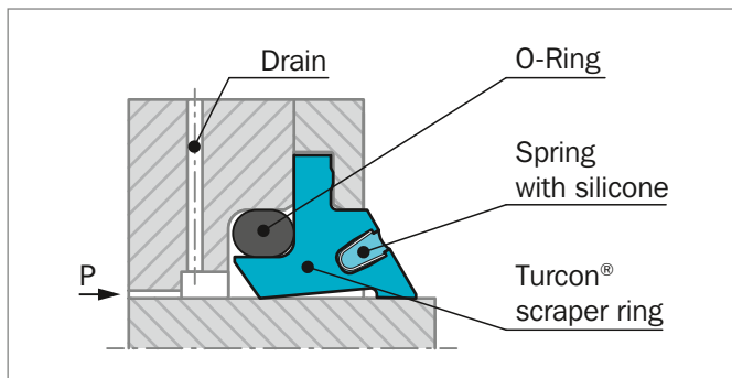
Figure 168: Turcon® Excluder® S with V-Spring activated lip
