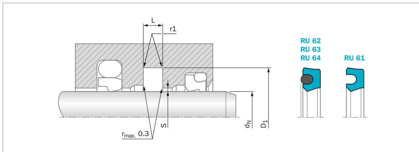
Figure 51: Installation Drawing
