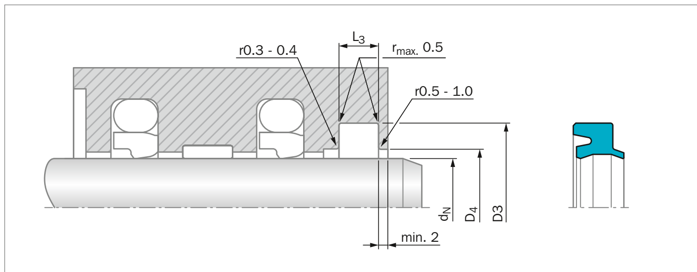
Figure 182: Installation Drawing
